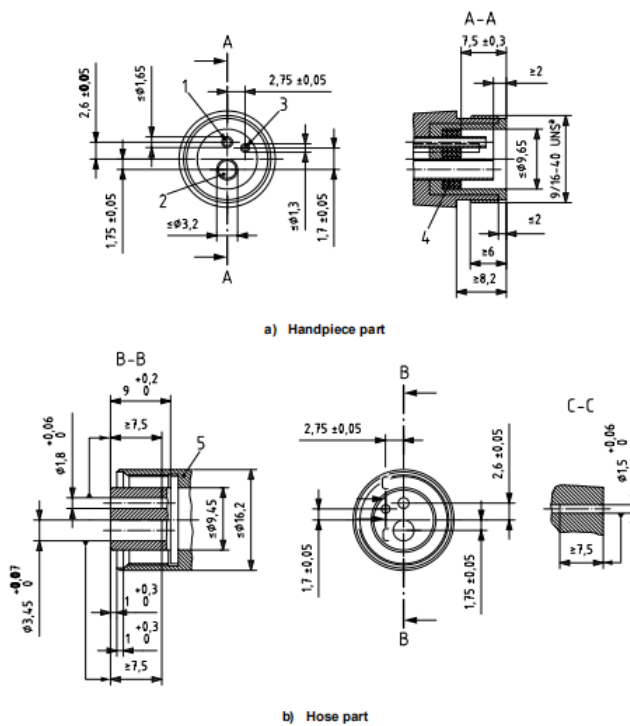
Figure 4: handpiece hose part of type 1 connector
